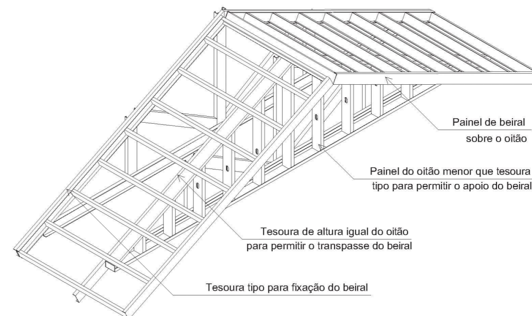
Figura 5.20 - Painel de beiral
